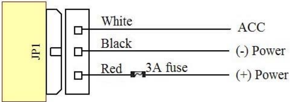
Wiring diagram
